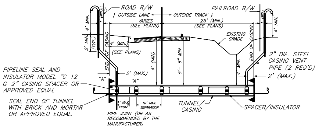
SECTION "A"
