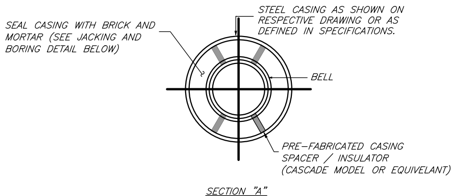
SECTION "A"
